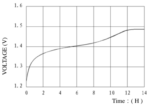
TYPICAL CHARGE CURVE (1.3mA)
