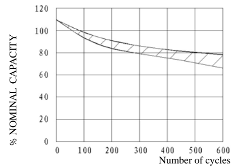
CYCLE LIFE CURVE
