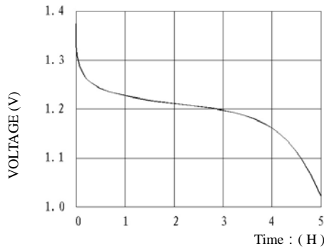
TYPICAL DISCHARGE CURVE (2.6mA)
